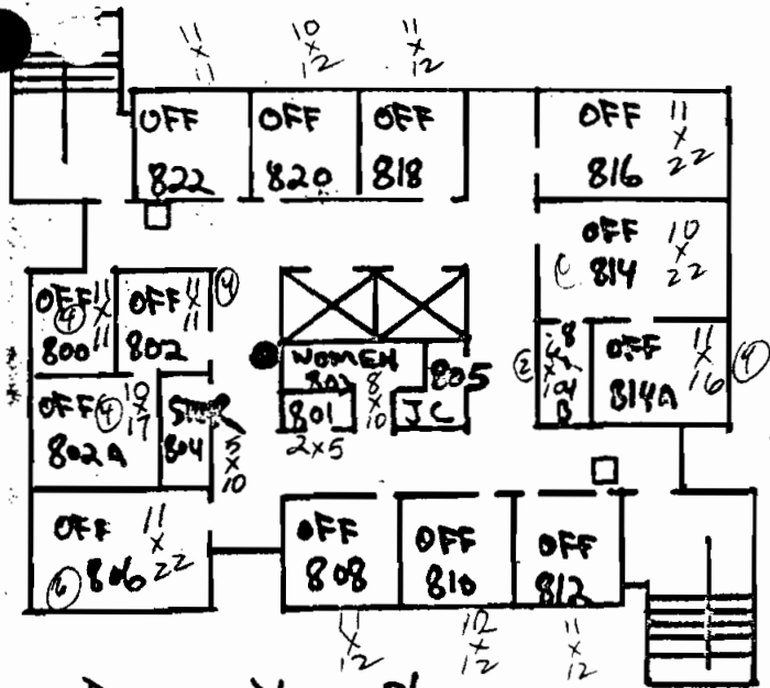
EIGHTH Floor PLAN
